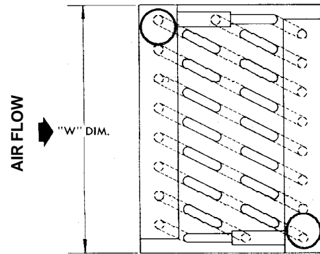
6 ROW KWS CIRCUITING HORIZONTAL OR VERTICAL AIR FLOW
