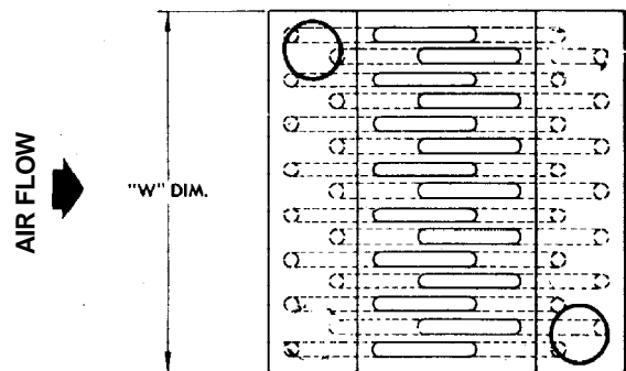
8 ROW KWD CIRCUITING HORIZONTAL OR VERTICAL AIR FLOW
