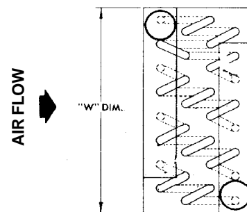
4 ROW KWH CIRCUITING HORIZONTAL OR VERTICAL AIR FLOW
